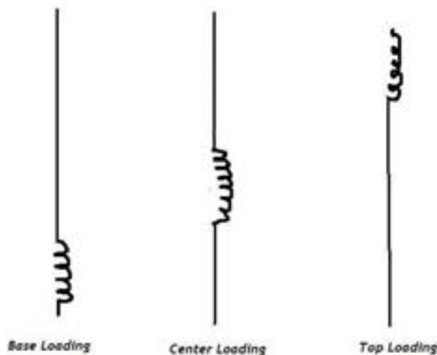
Figure 2: A loading coil usually is added at base, sometimes center or top, of a short vertical. (Drawing by author)
