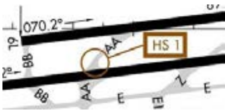
An example of how a hot spot is depicted on an airport diagram. (Courtesy: FAA)
