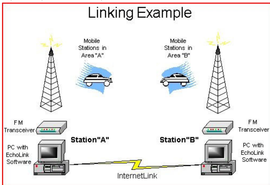
How Echolink works. (Courtesy: Echolink.org)
