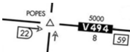
Chart example of an intersection. The POPES intersection is defined by the Santa Rosa VOR (STG) 077 degree radial crossing the Scaggs Island VOR (SGD) 349 degree radial and also where Route V494 crosses Route V87. Look up POPES using SkyVector to see it in the larger context (Enroute L-2 and L-3 charts).
